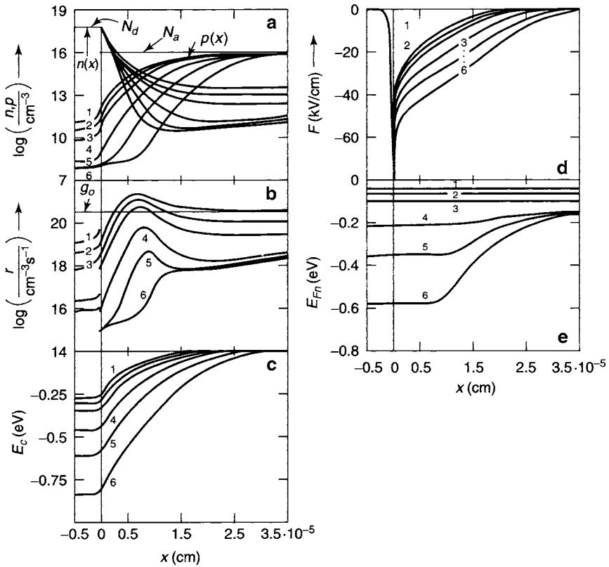
Fig. 10.22. Solution curves for a thin, asymmetrically doped Si pn -junction with the net current as family parameter for j = 150, 0, -29, -34.5, -35 , and 35.6 \text{ mA cm}^{-2} for curves 1–6, respectively.
