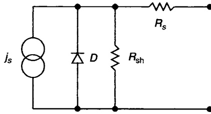
Fig. 8.6. Simple equivalent circuit of a solar cell diode D with series and shunt resistances identified
